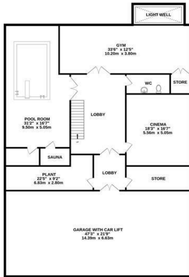
LOWER GROUND FLOOR 3083 sq.ft. (286.4 sq.m.) approx.
